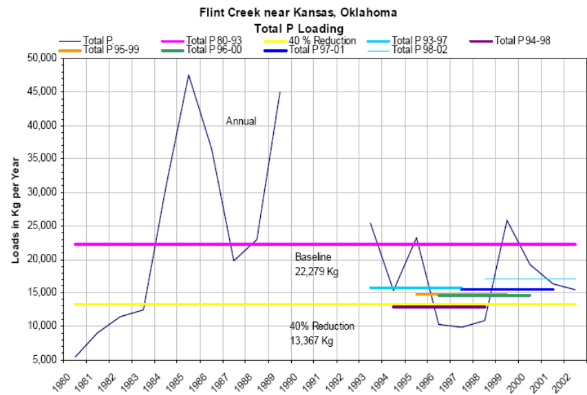
Figure 8. Total phosphorus trends at Oklahoma sites from 1980 to 2002.
