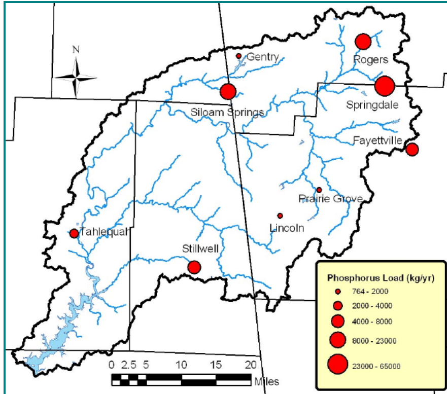
Figure 9. Total phosphorus loads from Waste Water Treatment Plants with a significant discharge in the Illinois River basin (Storm et al. 2006).
