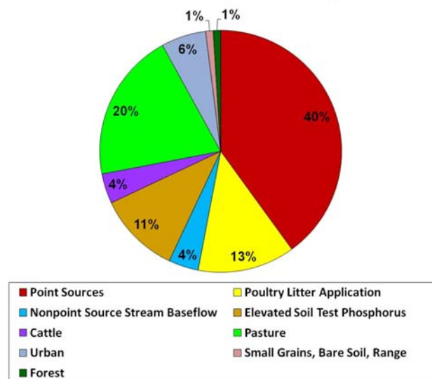
Figure 16. Total phosphorus reaching Lake Tenkiller by source as predicted by SWAT with new in-stream model (1990-2006) (from Storm et al. 2010).
