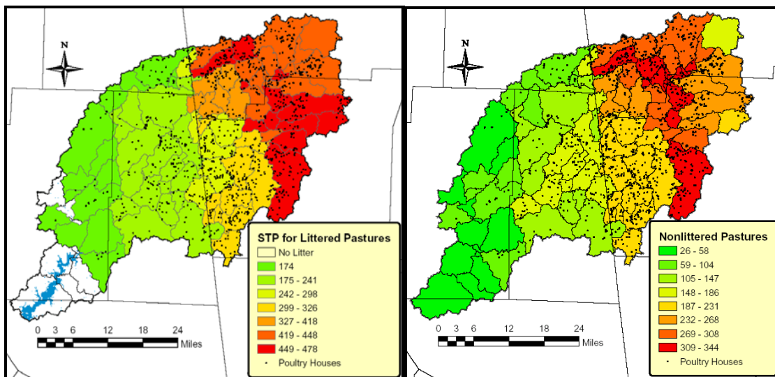
Figure 12. Estimated average soil test phosphorus for pastures a) receiving poultry waste (litter) and b) not currently receiving poultry waste (“litter”) (Storm et al. 2006). Note: the STP values corresponding to specific colors are different in the two graphics—refer to the key.
