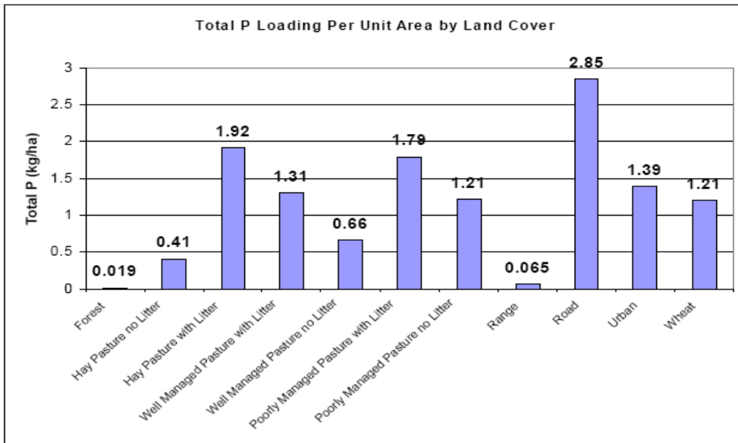
Figure 14. Total phosphorus load per unit area as predicted by the SWAT and instream models in the Illinois River basin (Storm et al. 2006).
