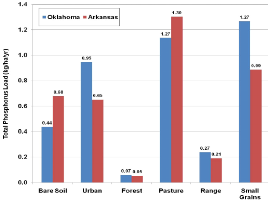
Figure 17. Upland total phosphorus load per unit area by land cover and by state as predicted by the SWAT model in the Illinois River basin (1990-2006) (from Storm et al. 2010).
