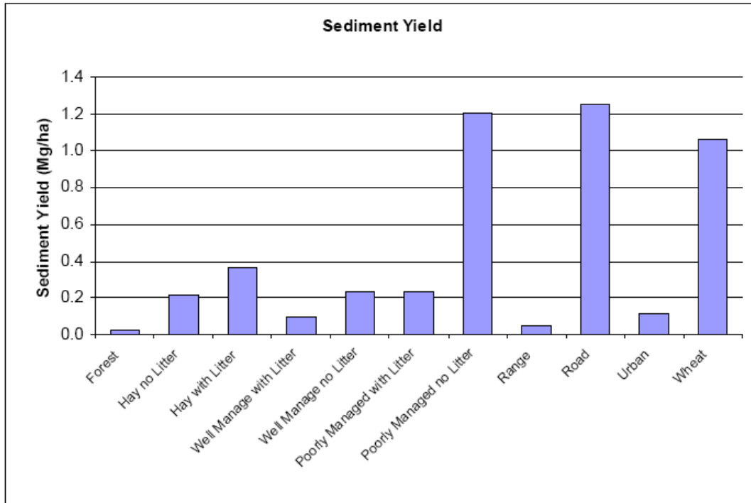
Figure 15. Sediment yield per unit area by source as predicted by the SWAT and instream models in the Illinois River watershed (Storm et al. 2006).
