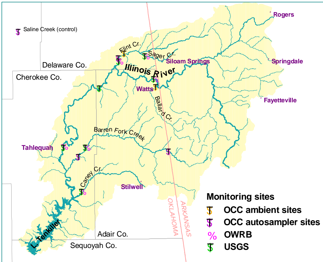
Figure 21. Monitoring sites in the Illinois River watershed.
