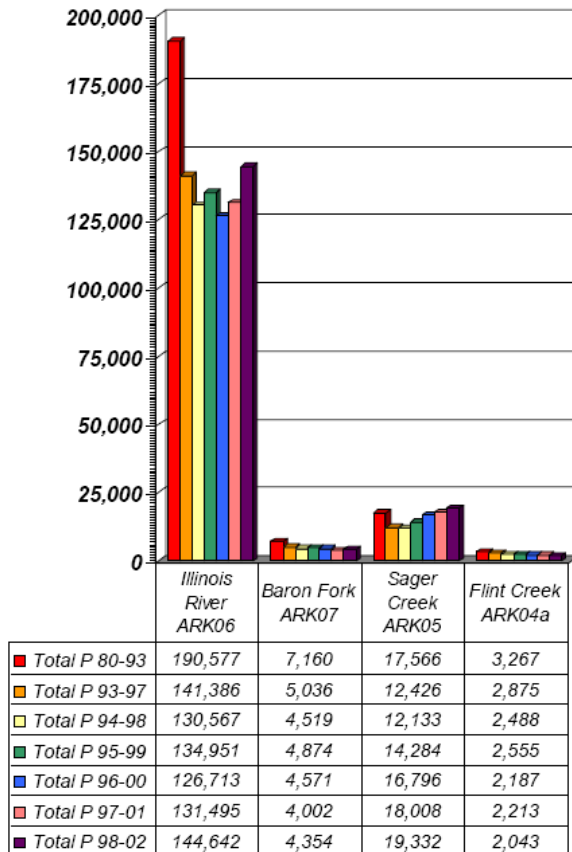
Figure 7. Average annual total phosphorus (kg/yr) at Arkansas sites (left) and Oklahoma sites (right) from 1980 to 2002.
