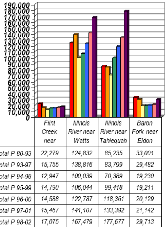
Figure 7. Average annual total phosphorus (kg/yr) at Arkansas sites (left) and Oklahoma sites (right) from 1980 to 2002.
